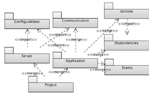
Fig. 1. Logical packages and dependencies of the BOINC functionalities
